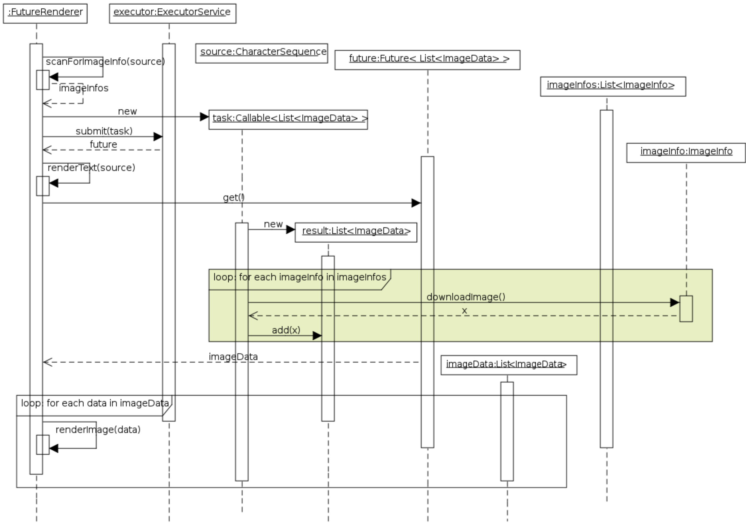
sequencediagram for renderPage(CharSequence source) method of FutureRenderer class
